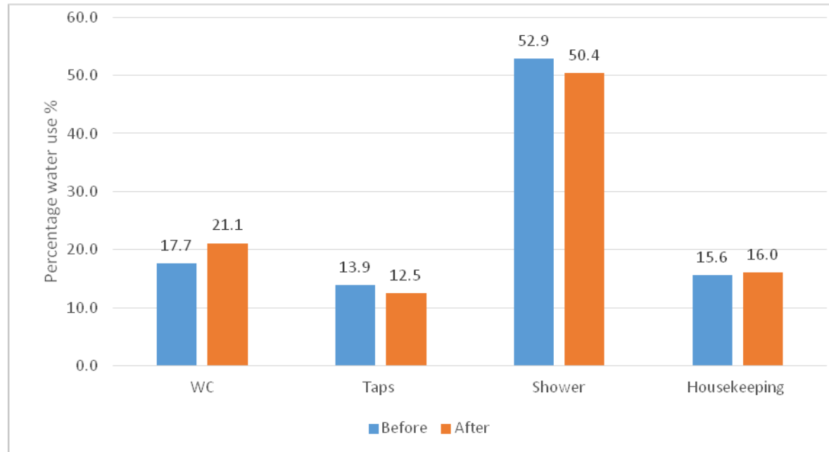
Figure 2: Percentage breakdown of water use in guestrooms, showing before and after the retrofits
