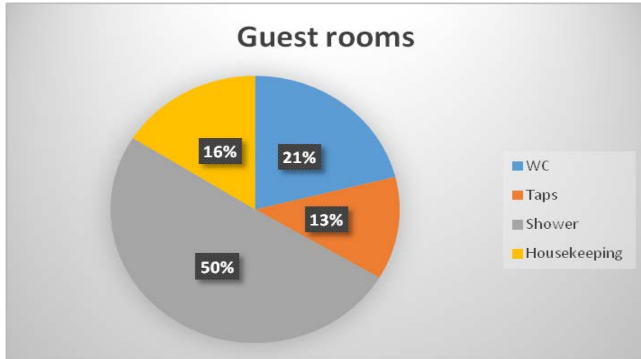
Figure 3: Percentage breakdown of water use in guest rooms post-retrofit (first quarter)
